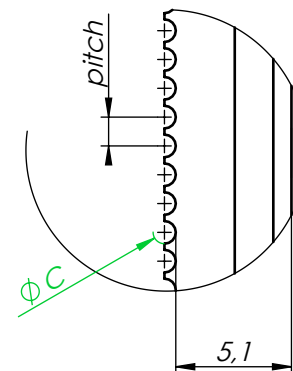
DETAIL B SCALE 3 : 1
