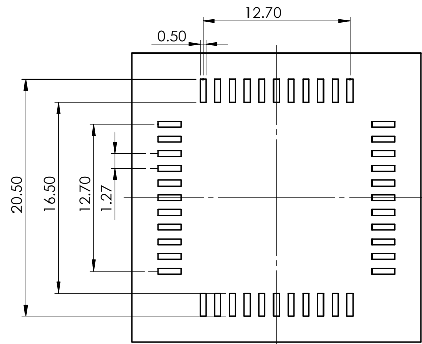
PCB LAYOUT
