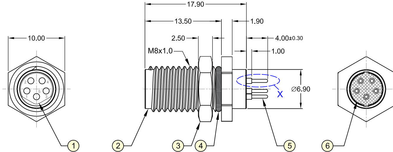
Detail X
